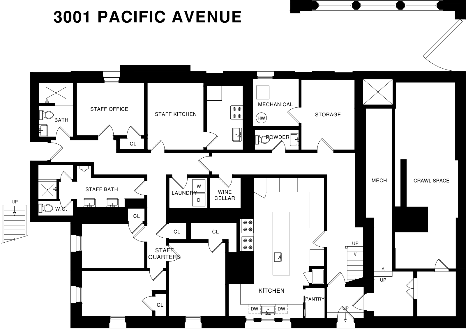
BASEMENT LEVEL
